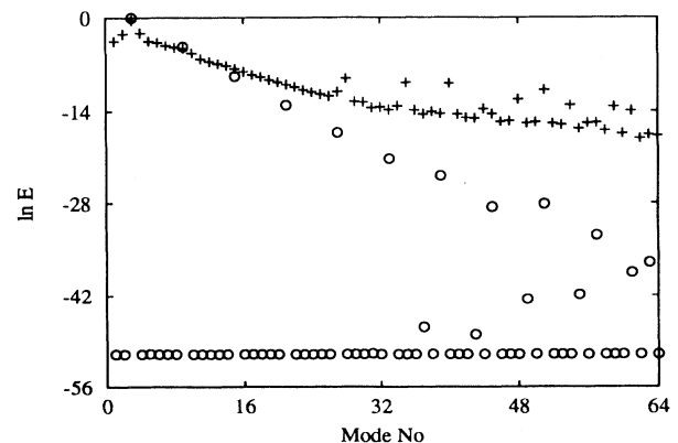
FIG. 2. Natural logarithm of mode energy for E=3.0 and N=64 and initial energy in mode 3 (circles) and 90% in mode 3 (pluses).
